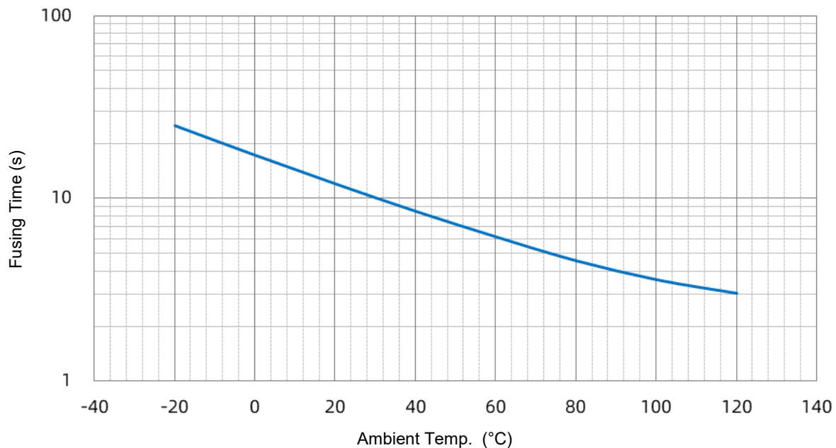
SHP 45 A Temp.-Time Curve
